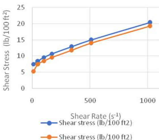
Fig. 10. Shear stress Vs shear rate curve for runorder4
