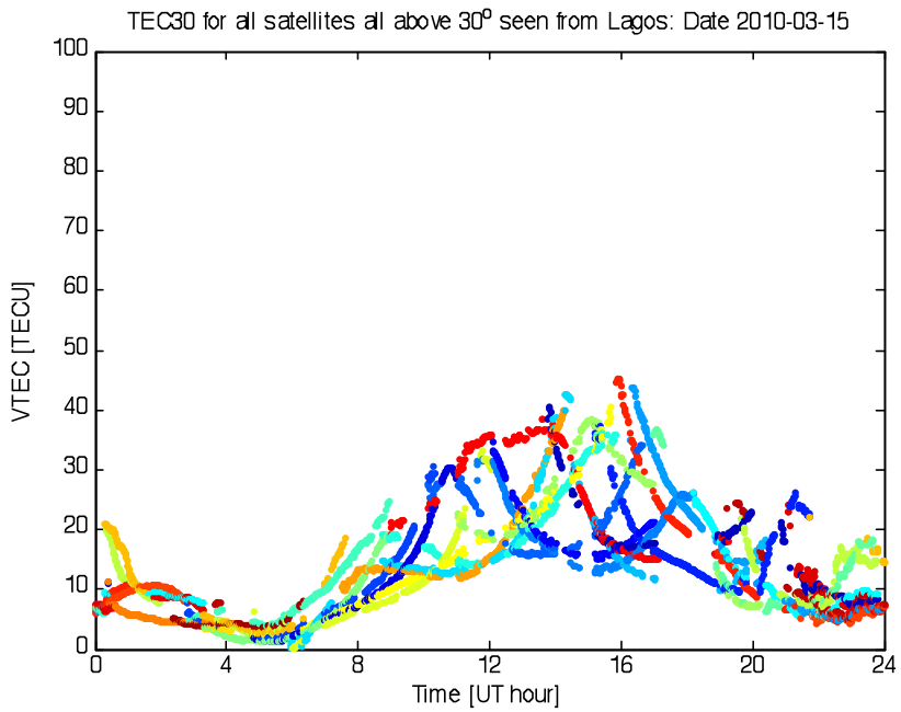
Figure 4.2.4: Plots of (a) S_4 (b) sigma (c) TEC (d) TEC rate for 15 March 2010 (LT = UT + 1h)
