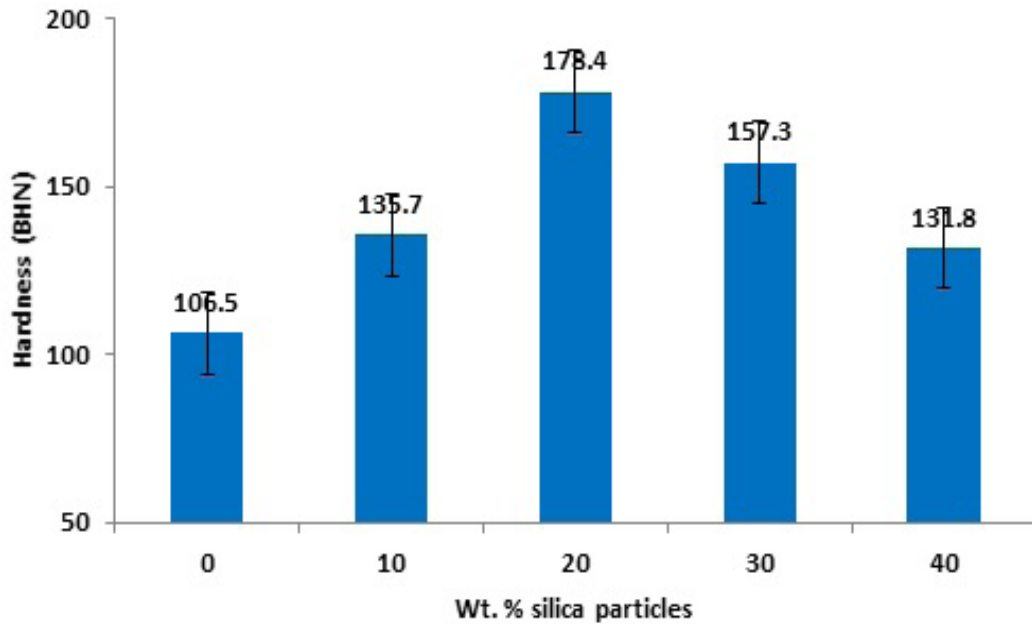
Fig. 7: Variation of hardness with silica particles addition
