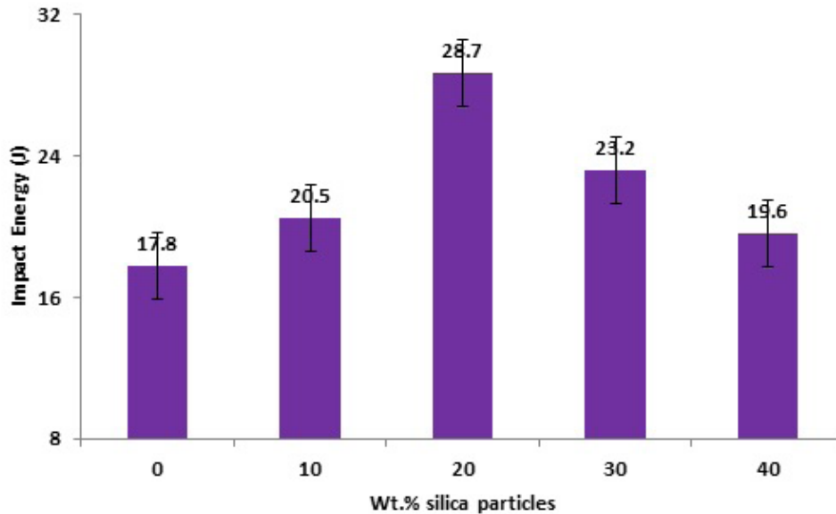
Fig. 8: Variation of impact energy with silica particles addition
