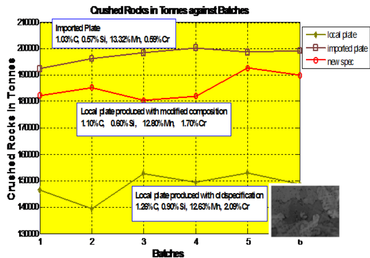
Figure 2. Comparative Output of Crushed Rock for Three Compositions: (b) Micrograph of old spec
