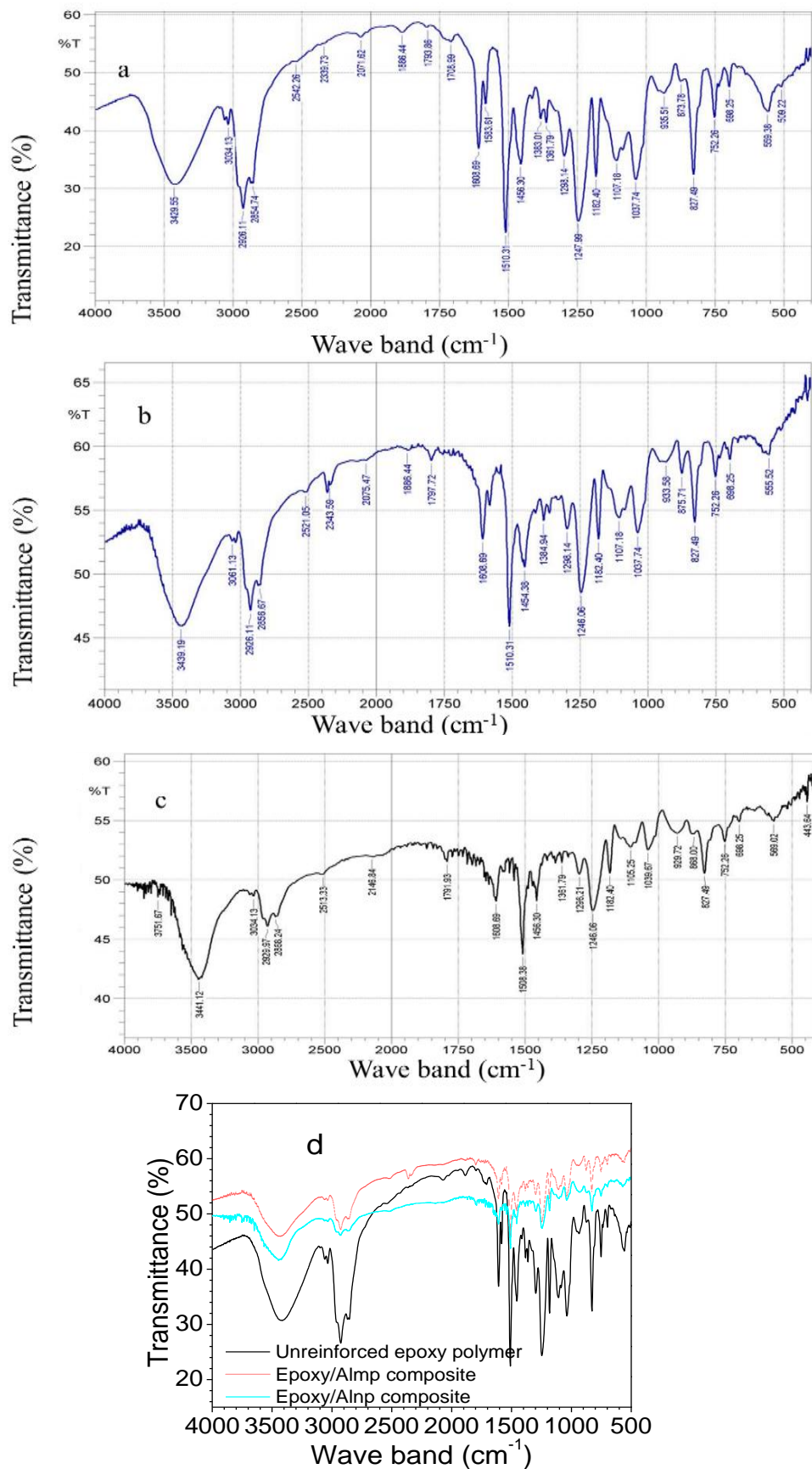
Fig. 2. Bond characteristics of (a) epoxy polymer; (b) epoxy/Alnp; (c) epoxy/Alnp composites; (d) superimposed FTIR spectra of all samples.
