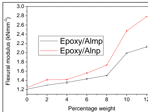
Fig. 6. Flexural modulus of epoxy/aluminium composites.
