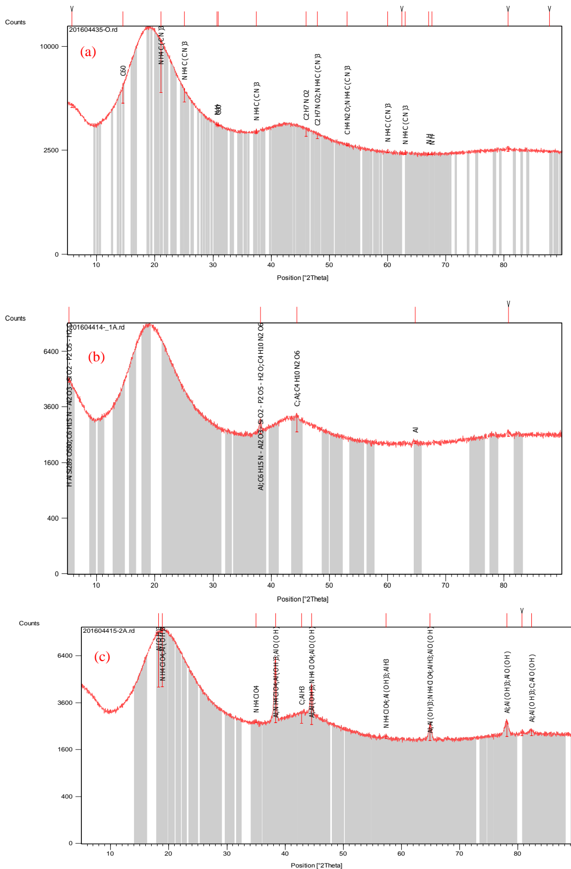
Fig. 3. X-ray diffractograms of (a) epoxy polymer; (b) epoxy/Almp; (c) epoxy/Alnp composites.
