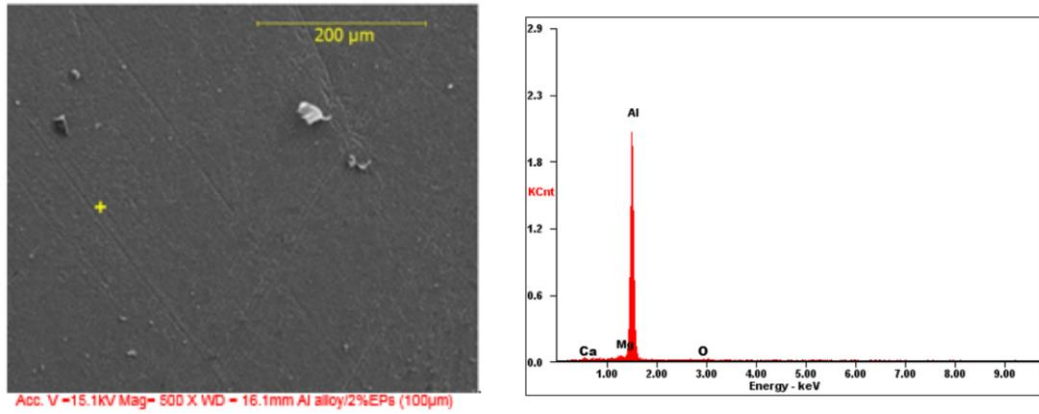
Fig 3: SEM/EDX of Al alloy/2% ESp (100µm) composites
