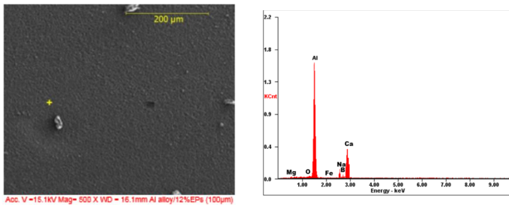
Fig 5: SEM/EDX of Al alloy/12% ESp (100µm) composites
