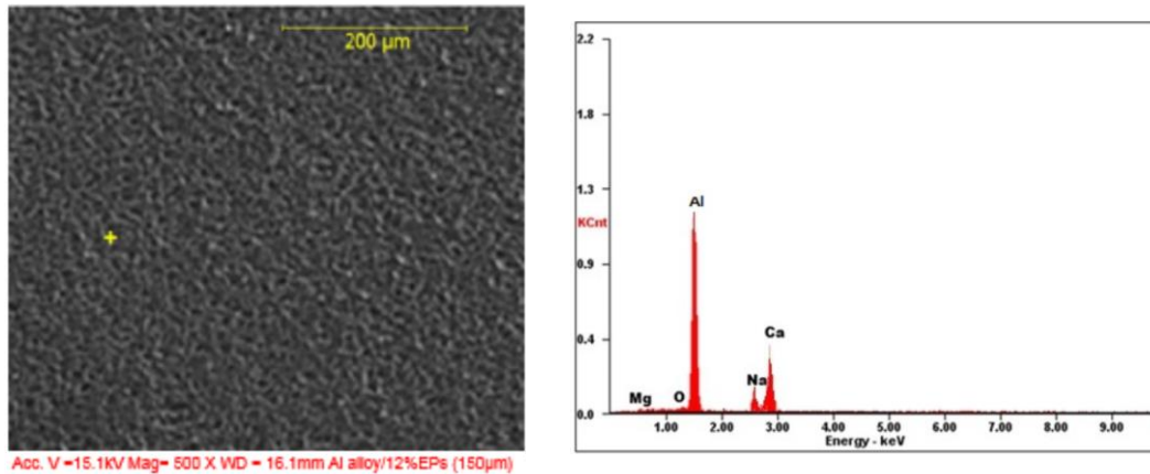
Fig 6: SEM/EDX of Al alloy/12% ESp (150µm) composites
