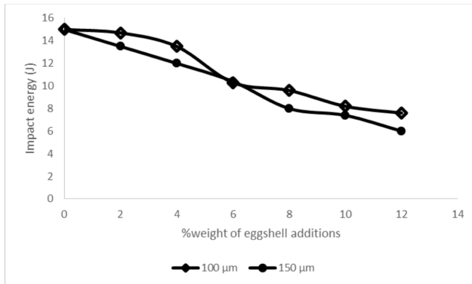
Fig 10: Impact of Al alloy/ESp composites with wt. % of ESp additions
