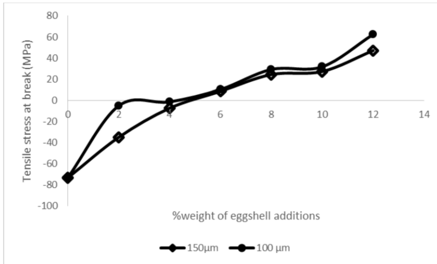
Fig 7: Fracture stress of Al alloy/ESp composites with wt. % of EPs additions
