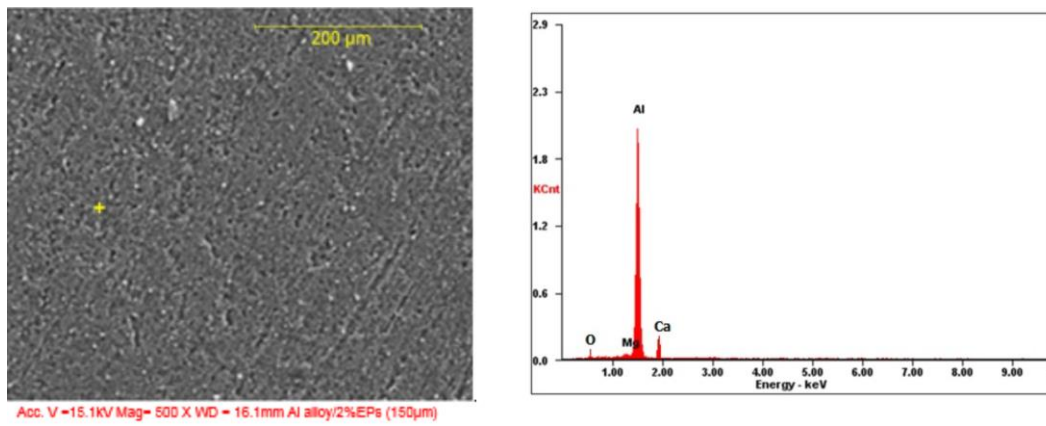
Fig 4: SEM/EDX of Al alloy/2% ESp (150µm) composites
