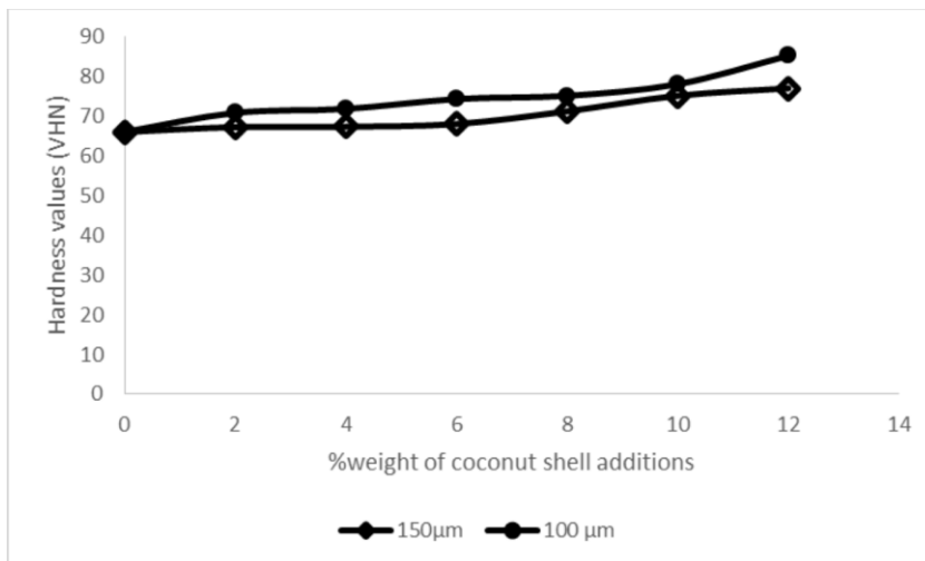
Fig 8: Hardness values of Al alloy/ESp composites with wt. % of EPs additions
