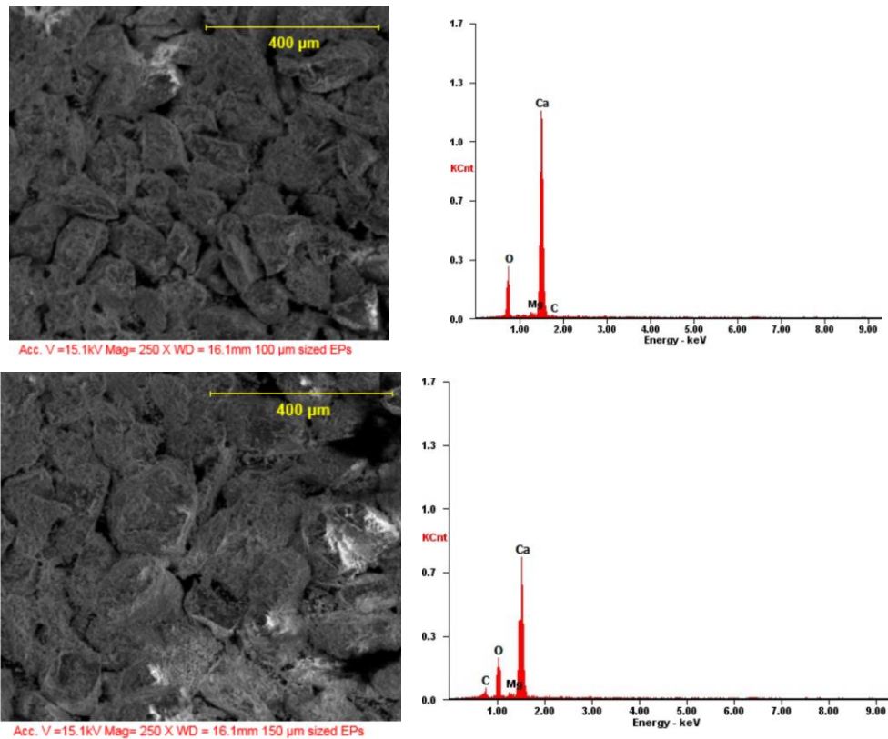
Fig 1: SEM/EDX of the \text{CaCO}_3 particles (a) 100 µm; (b) 150 µm
