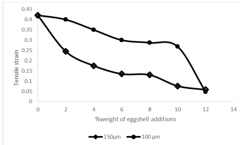
Fig 9: Tensile strain of Al alloy/ESp composites with wt. % of EPs additions
