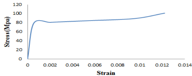
Figure 9: Henry Schein Stress strain behaviour under three point loading
