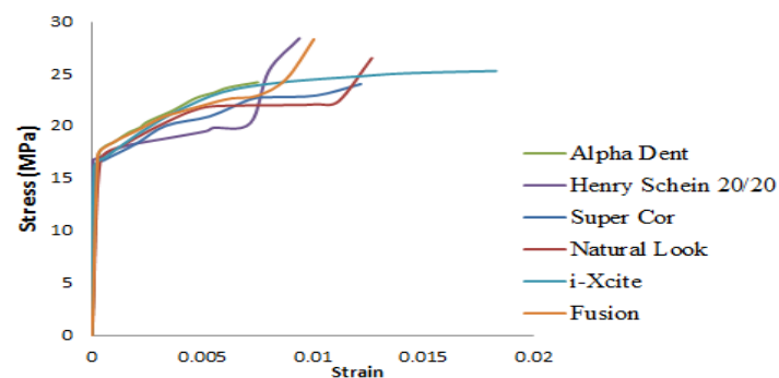
Figure 7: Stress strain behaviour of all samples under tensile loading
