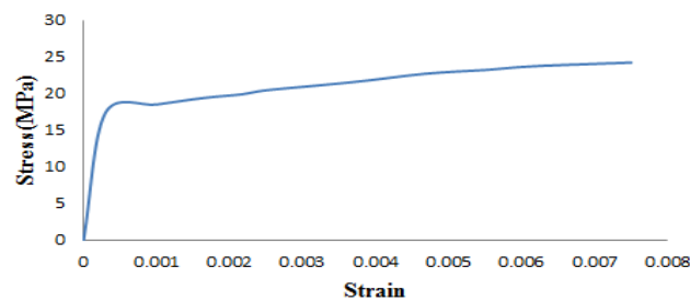
Figure 1: Alpha Dent Stress strain behaviour under tensile loading
